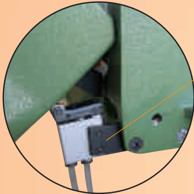
MICROVALVOLA per apertura e chiusura morse MICROVALVE for the opening and the closing of the clamps
